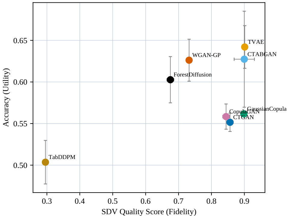
Mushroom: SDV Quality Score (Fidelity) vs Accuracy (Utility)
